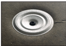
Incorrectly installed, overdriven plate/fastener.
